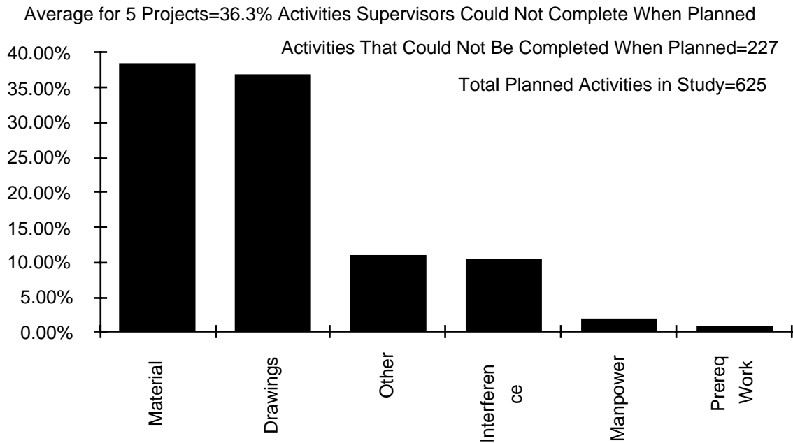
Figure 3: Construction last planner: Comparing 'should' with 'did.'
